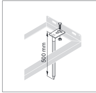
Optional Bodenanker (2er-Set). Optional ground tie-bolts, galvanised (set of 2).
