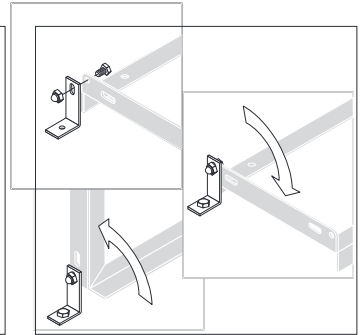
Optional Bodenmontage- Winkel, verzinkt (2er-Set). Optional galvanised floor- mounting bracket (set of 2). Art.-Nr. Item No. 105800002
