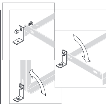
Bodenmontage-Winkel, verzinkt (2er-Set). Floor mounting bracket, galvanised (set of 2).
